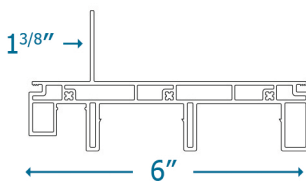
PD1901 FRAME HEAD AND JAMB
